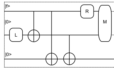
Figure 8: Inappropriate circuit.
