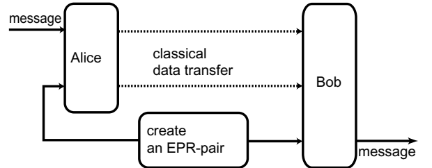
Figure 1: Idea of quantum teleportation.
