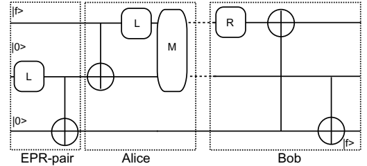
Figure 3: Evolved circuit for teleportation.
