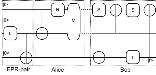
Figure 2: Brassard's circuit (Brassard, 1996).
